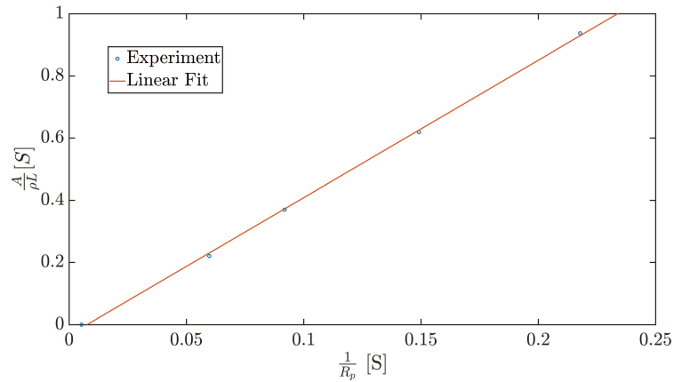
Figure B.5: Calculated free flow conductance as a function of the electric conductance in Whatman #1 substrate. Constriction factor ( C ) can be obtained from the slope of the linear fit, according to Eq. (B.10).
