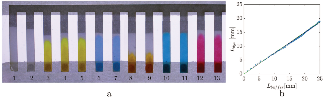
Figure C.4: Paper-based chromatography of multiple dyes a) Screenshot of the chromatography experiment for selected dyes at t=180 s and \text{pH}=5.5 . 1-2 are control strips, filled with buffer. 3-5 Tartrazine, 6-7 Brilliant Blue, 8-9 Methyl Orange, 10-11 Fast Green, and 12-13 Red Ponceau. b) Linear fit of Tartrazine and buffer front positions. The slope of this line is the retardation factor R_f .
